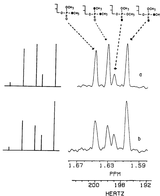
Figure 7. Calculated and observed ^{31}\text{P} NMR spectra of 12 (a) and 14 (b) (in \text{CDCl}_3 ) obtained from [\text{^{17}O, ^{18}O}] DPPE 4. Spectral parameters are the same as in Figure 5.
