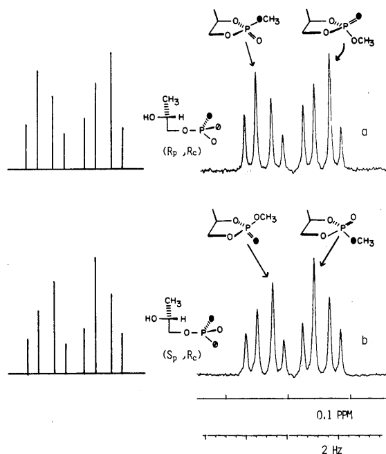
Figure 10. ^{31}\text{P} NMR spectra (at 121.47 MHz) of the mixtures of syn and anti cyclic triesters (in \text{CD}_3\text{CN} ) derived from [ ^{16}\text{O} , ^{17}\text{O} , ^{18}\text{O} ]phospho-( R )-propane-1,2-diols. (a) From isomer 3 of [ ^{17}\text{O} , ^{18}\text{O} ]DPPE; (b) from isomer 4 of [ ^{17}\text{O} , ^{18}\text{O} ]DPPE. Spectral parameters: spectral width 500 Hz; 16 K data points; ^1\text{H} decoupling; 90^\circ pulse; line broadening 0.2 Hz; chemical shift +19.7 ppm; temperature 25^\circ\text{C} . The calculated spectra are shown on the left side.
