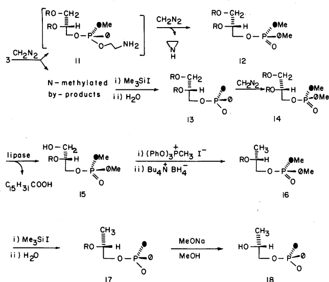
Figure 6. Conversion of (R_p) - [\text{^{17}O, ^{18}O}] DPPE (3) into 1- (R_p) - [\text{^{16}O, ^{17}O, ^{18}O}] phospho- (R) -propane-1,2-diol (18). R = \text{C}_{15}\text{H}_{31}\text{CO} ; ^{18}\text{O} = \bullet ; ^{17}\text{O} = \emptyset .
