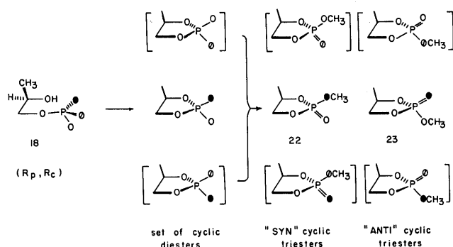
Figure 9. Ring closure and methylation of 1-( R p )-[ ^{16}\text{O} , ^{17}\text{O} , ^{18}\text{O} ]phospho-( R )-propane-1,2-diol (18), according to the procedure of Abbott et al., 15 except that the configuration of \text{C}_2 is different.
