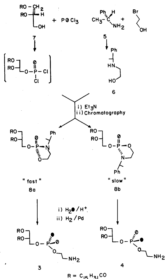
Figure 2. Synthesis of (R p )- and (S p )-[17O, 18O]DPPE 3 and 4.
