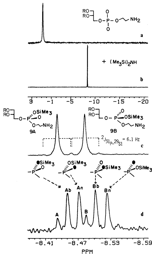
Figure 3. 31 P NMR analysis of DPPE and [18O]DPPE at 121.5 MHz. (a) DPPE (50 μmol) in CDCl 3 (2.5 mL): Spectral width 3000 Hz; acquisition time 2.7 s; 200 scans; line broadening 0.9 Hz. (b) DPPE (100 μmol) in CDCl 3 (2.5 mL), with addition of 50 μL HMDSA: spectral width 3000 Hz; acquisition time 2.7 s; 41 scans; line broadening -0.8 Hz; Gaussian broadening 0.07 Hz. (c) Same as (b): spectral width 500 Hz; acquisition time 16.4 s; 18 scans; line broadening -0.8 Hz; Gaussian broadening 0.07 Hz. (d) Randomly labeled [18O]DPPE plus HMDSA: same spectral parameters as (c). All spectra were taken at 25 °C, with 16 K data points and a 90° pulse (22 s).
